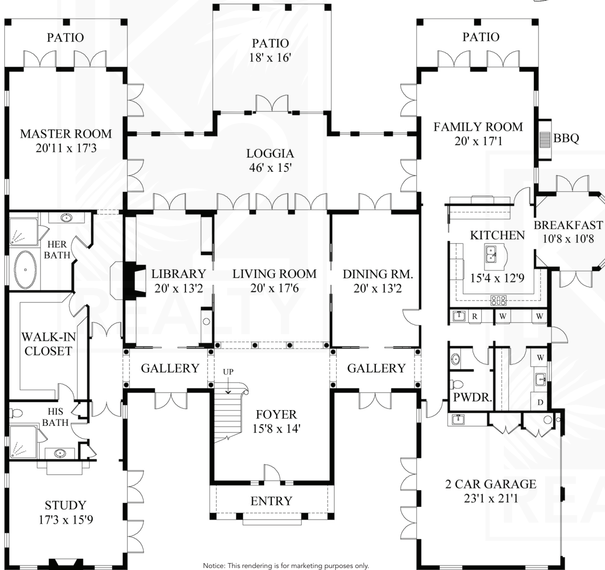
FIRST FLOOR
